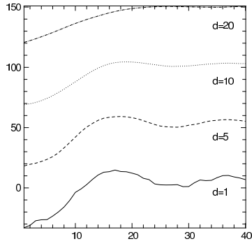
Fig. 5. Cross section through part of a wavefront averaged over discs of different diameter, d . The unit of length is taken to be the Fried parameter. The length of the segment is 40, the points are plotted a unit distance apart. The averaged values depend on the phases within a distance up to d/2 from the line segment.
