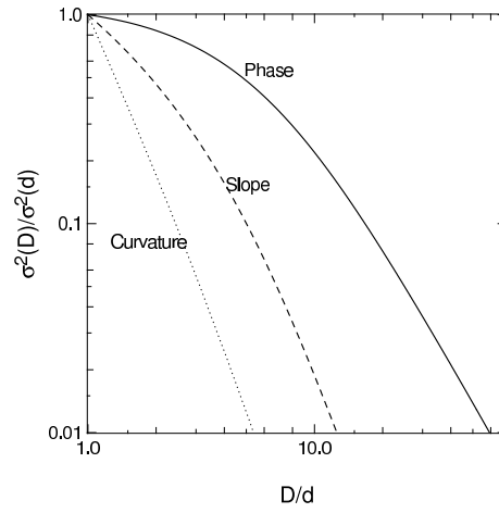
Fig. 7. Relative contribution of each layer to phase, slope and curvature measurements. The curves are calculated in terms of Eqs.5–7 with an outer scale L_0 = 10 m. The contribution of a distant layer ( D \gg d ) is smallest for curvature measurements.
